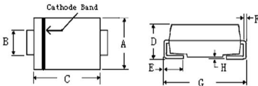
SMC/DO-214AB
