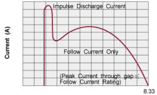
Period of Spark Gap Current (ms)
